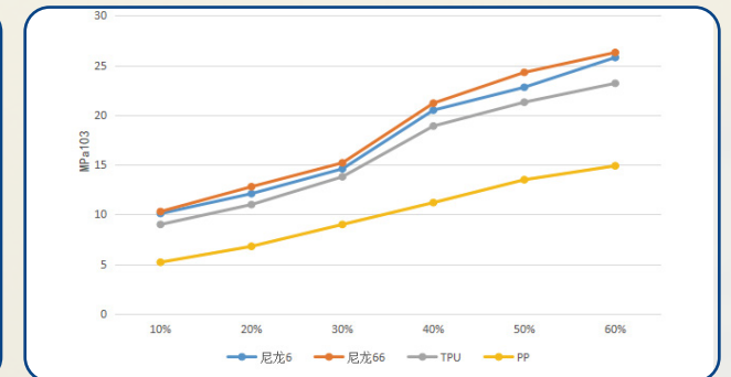
长碳纤增强多种塑料基材弯曲模量对比 Comparison of flexural modulus of various plastic substrates with long carbon fiber
