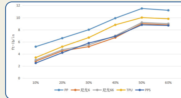
长玻纤增强多种塑料基材冲击性能对比 Comparison of impact property of various plastic substrates with long glass fiber
